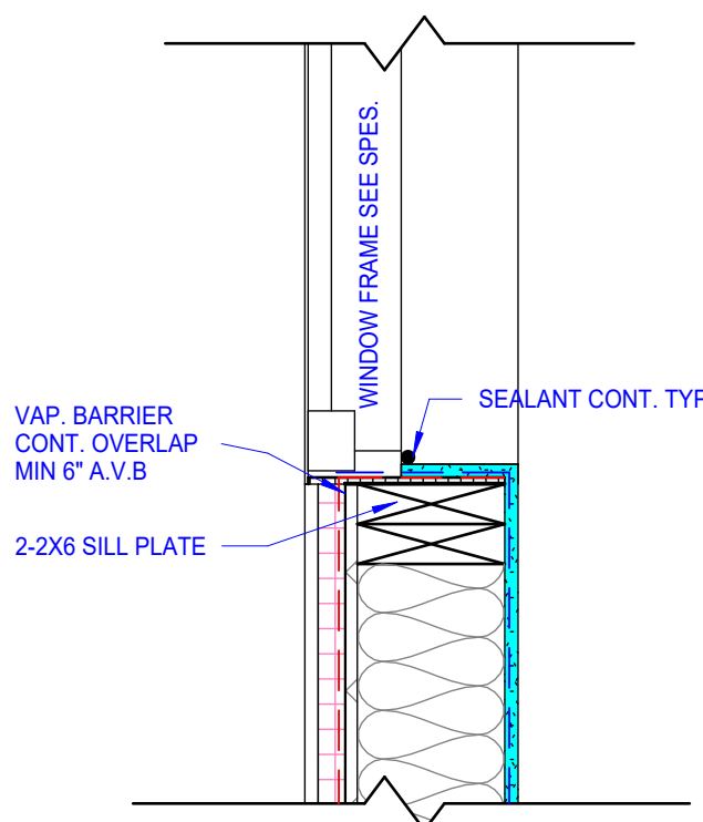
5 SILL DETAIL 1 1/2" = 1'-0"
