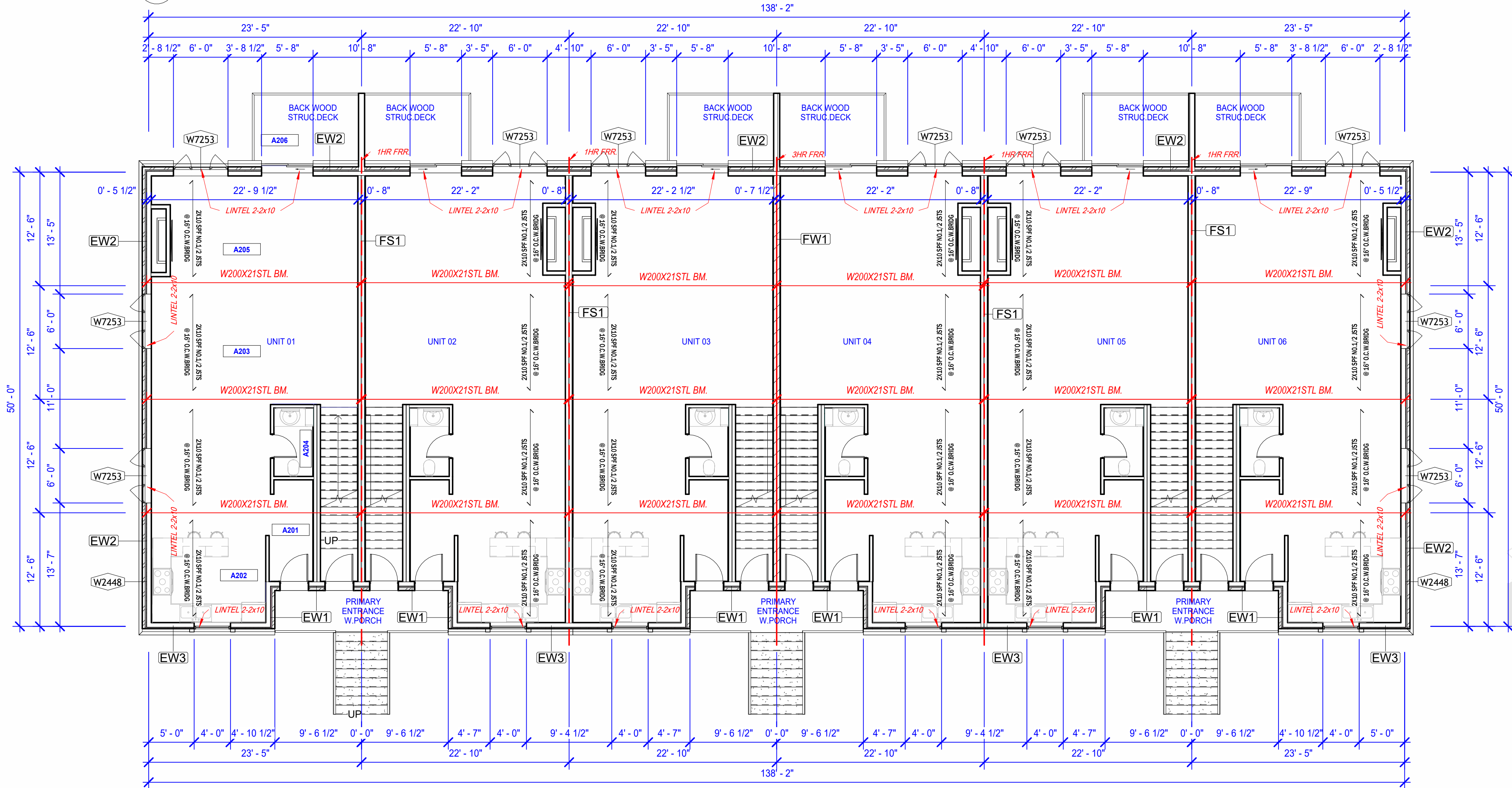
2 L200 - INTER. FLR. 1/8" = 1'-0"
