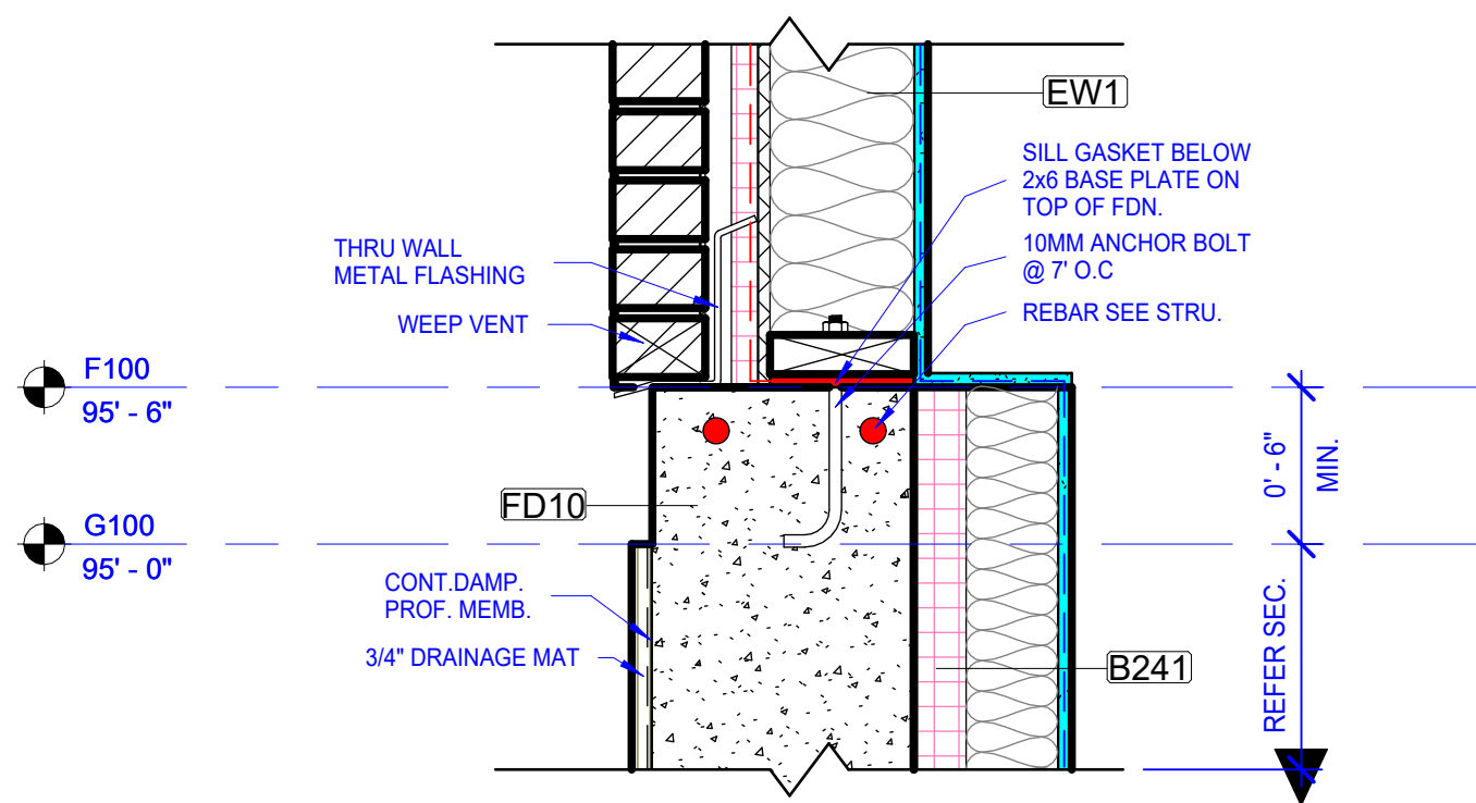
3 FDN. INTERSECTION DETAIL (TYP.) 1 1/2" = 1'-0"
