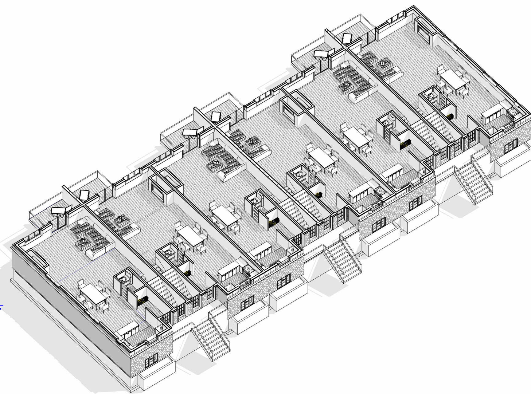
4 3D ISO L2
