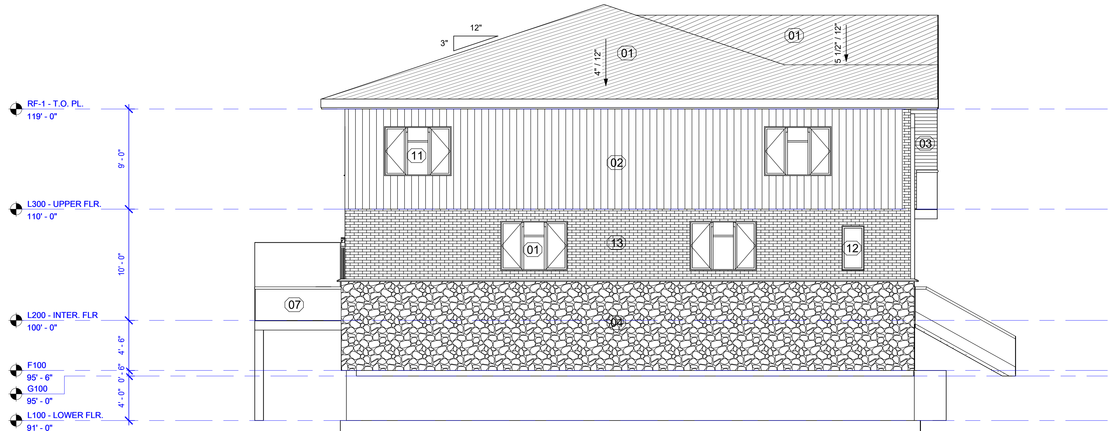
2 SIDE ELEVATION - RIGHT 3/16" = 1'-0"
