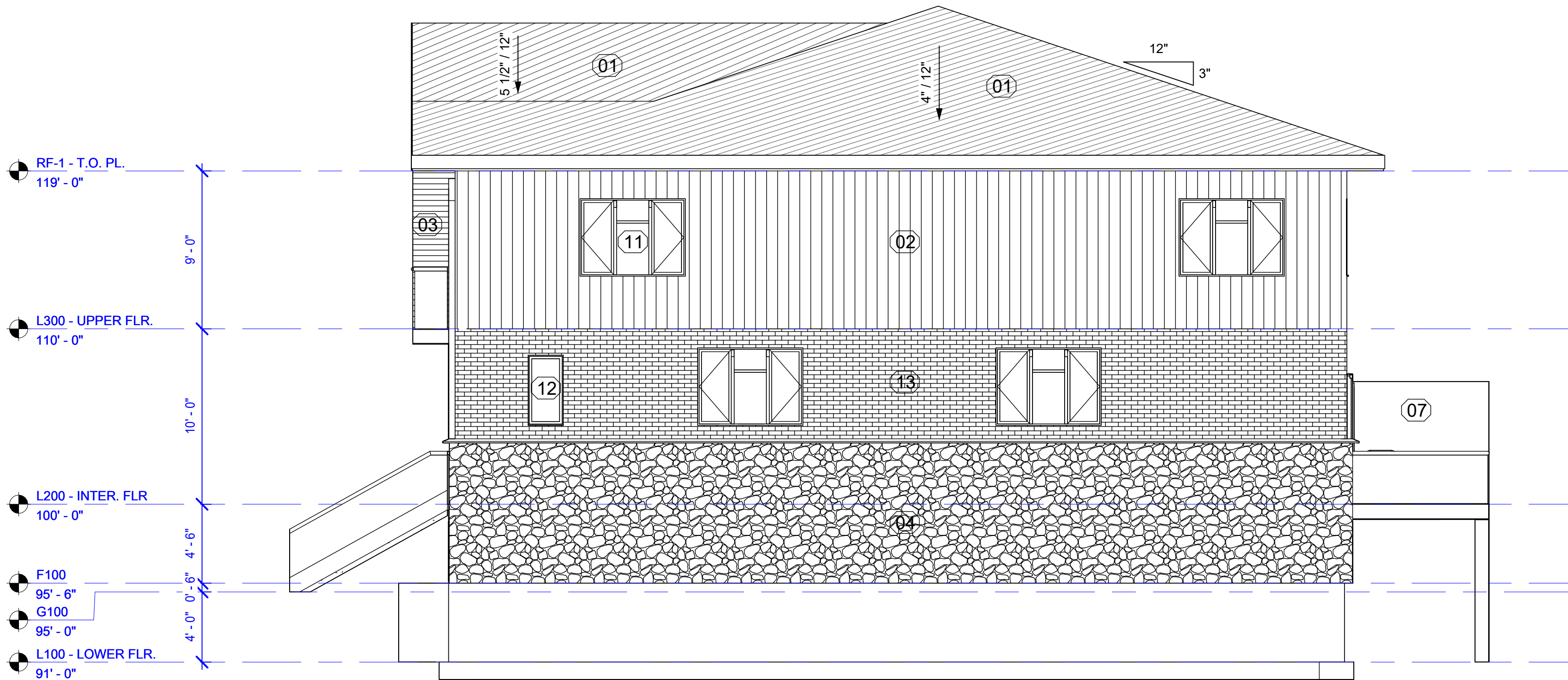
1 SIDE ELEVATION - LEFT 3/16" = 1'-0"
