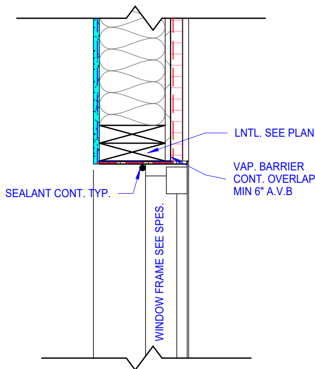
4 HEAD DETAIL 1 1/2" = 1'-0"
