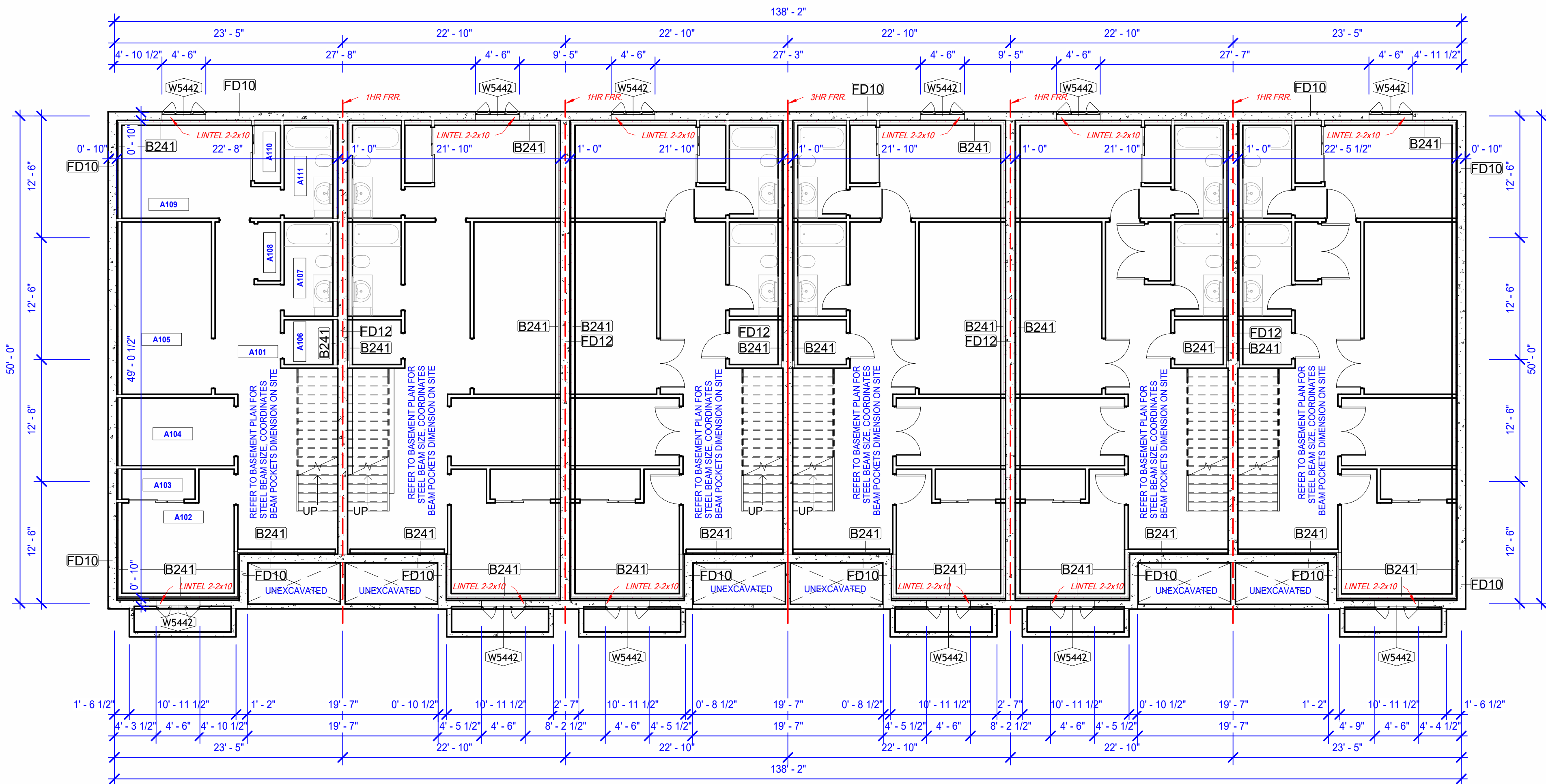
1 L100 - LOWER FLR. 1/8" = 1'-0"
