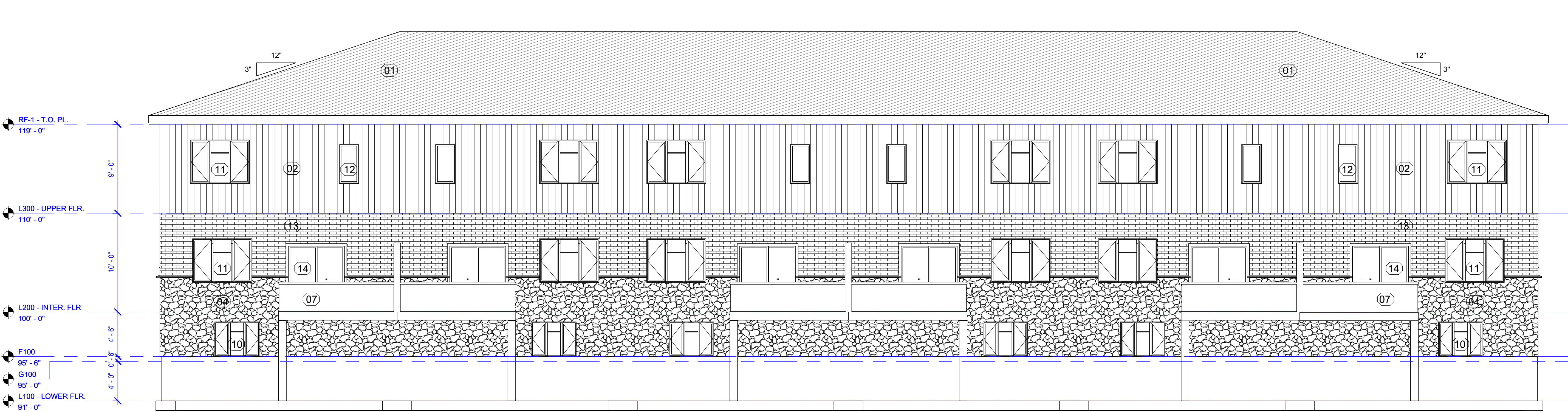
2 REAR ELEVATION 3/16" = 1'-0"
